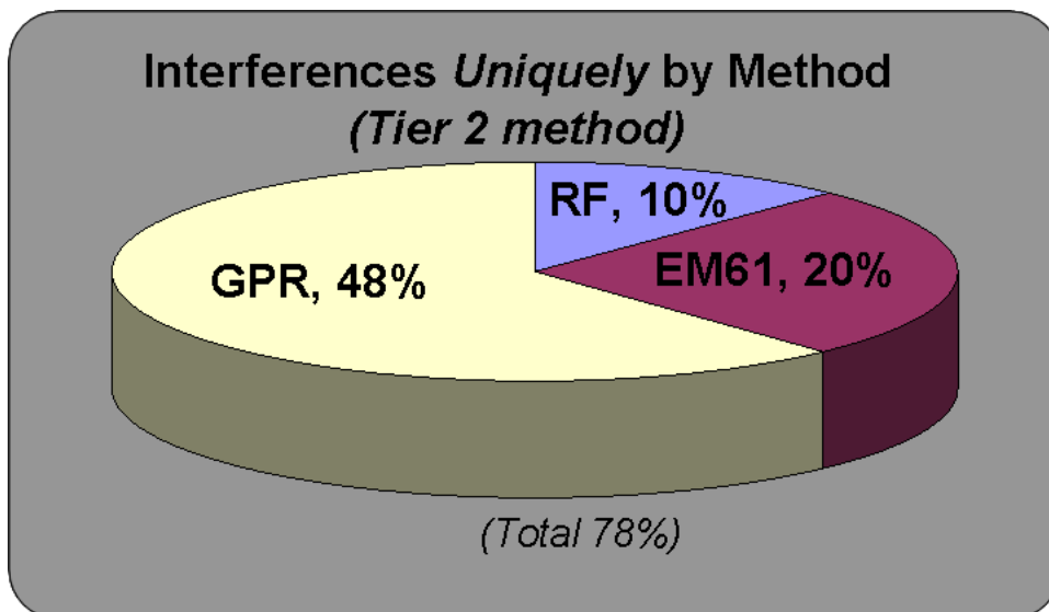
Figure 3. Pie chart showing the percentage of interferences uniquely designated by a given geophysical method for the same 23 Tier II surveys at the INL as shown in Figure 2. Note the sum of percentages here is only 78% as the interferences designated by more than one method were excluded. This result is worth noting in that it indicates that without the GPR mapping approach almost half the interferences would be missed by the survey. If only the GPR mapping were to be used, 30% of the interferences would have been missed (RF and EMI). This figure graphically illustrates the requirement for multiple methods to be used in subsurface surveying.
