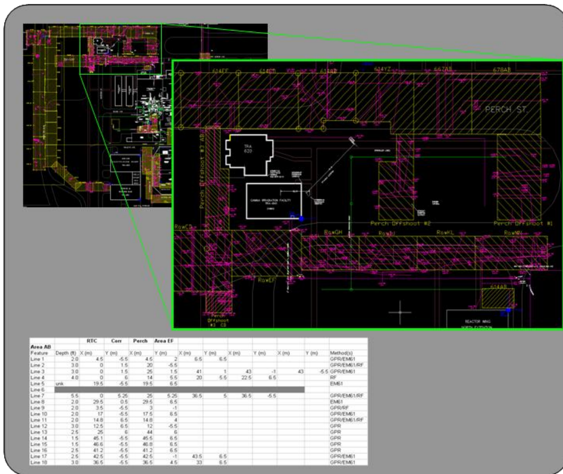
Figure 5. An example of a Subsurface Survey result in drawing form and a listing of the interferences designated in one survey area from the drawing. Note the drawing includes nearby buildings and structures for reference, survey areas are marked in yellow and interferences in pink, the color used at the INL to designate unknown interferences.
