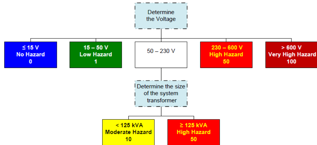
Chart 2 – ac, 60 Hz
