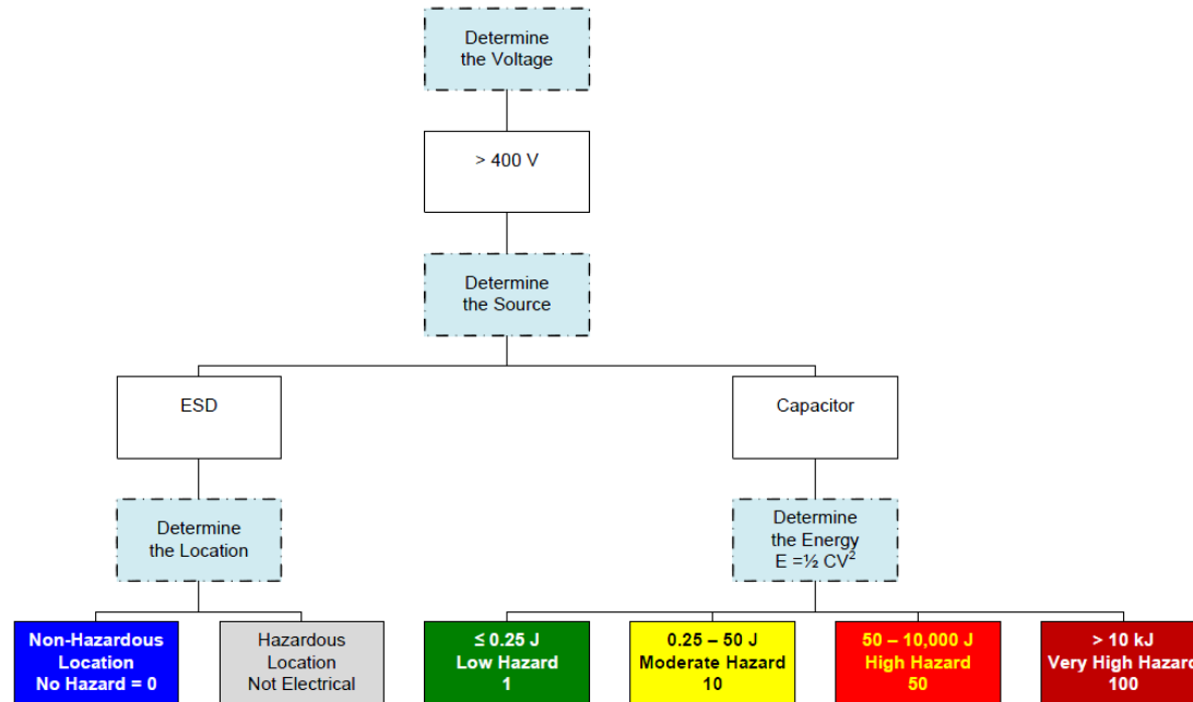
Chart 5 – Capacitors, > 400 V
