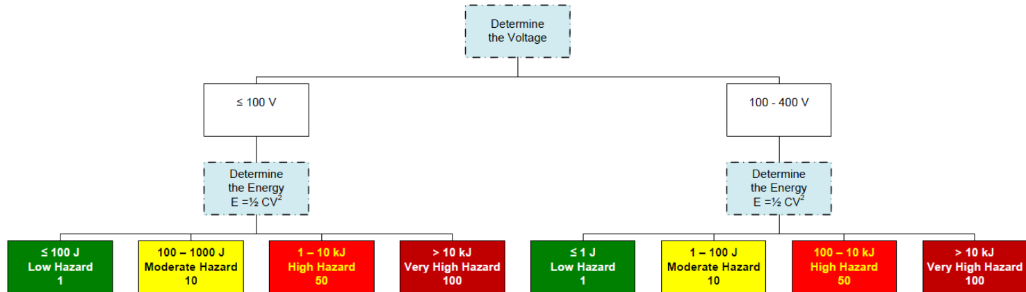
Chart 4 – Capacitors, < 400 V
