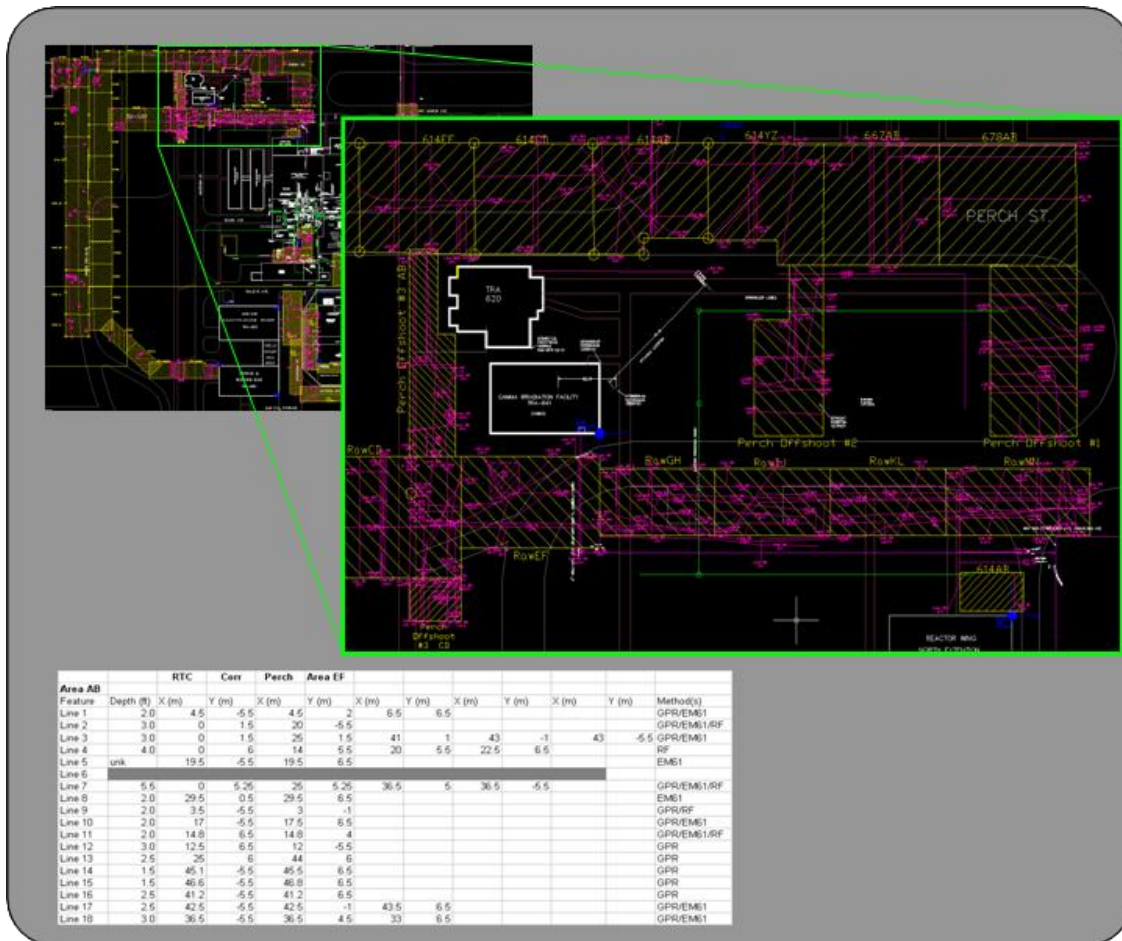
Figure 5. An example of a Subsurface Survey result in drawing form and a listing of the interferences designated in one survey area from the drawing. Note the drawing includes nearby buildings and structures for reference, survey areas are marked in yellow and interferences in pink, the color used at the INL to designate unknown interferences.
