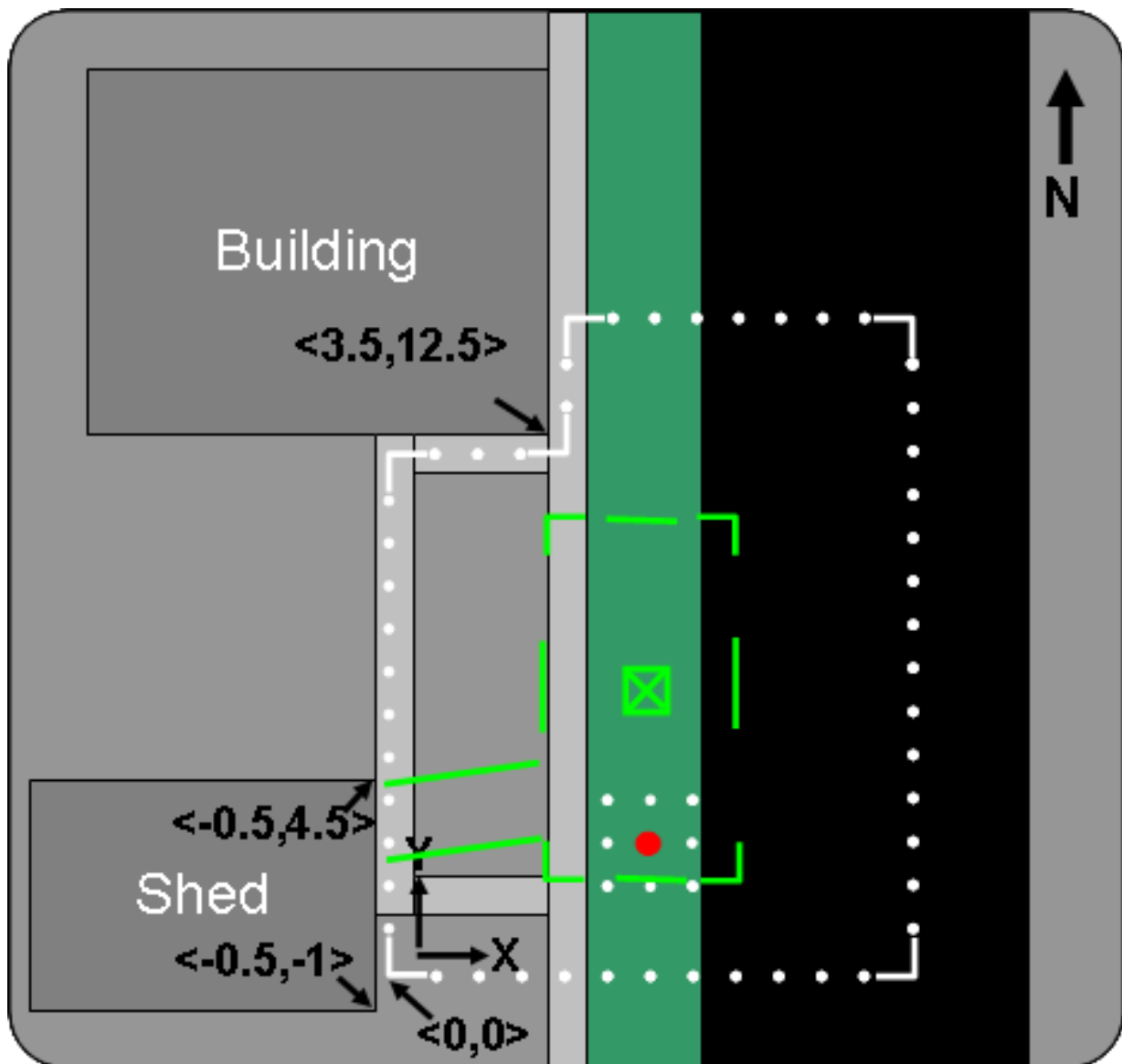
Figure 4. This sketch shows a map view of a typical 12 meter by 15 meter survey area near a building and a shed. Note this includes a cutout section around the building and what will be a
