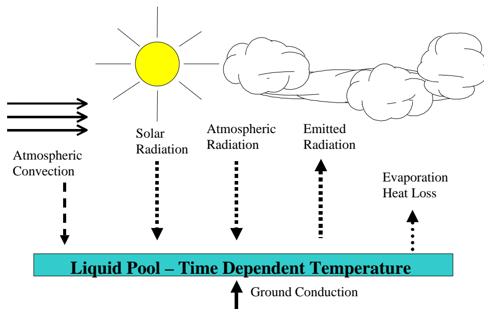
Figure 3. ALOHA Energy Balance for Evaporation Calculations.
